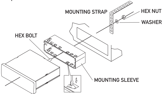
TYPICAL FRONT-LOAD DIN MOUNTING METHOD
